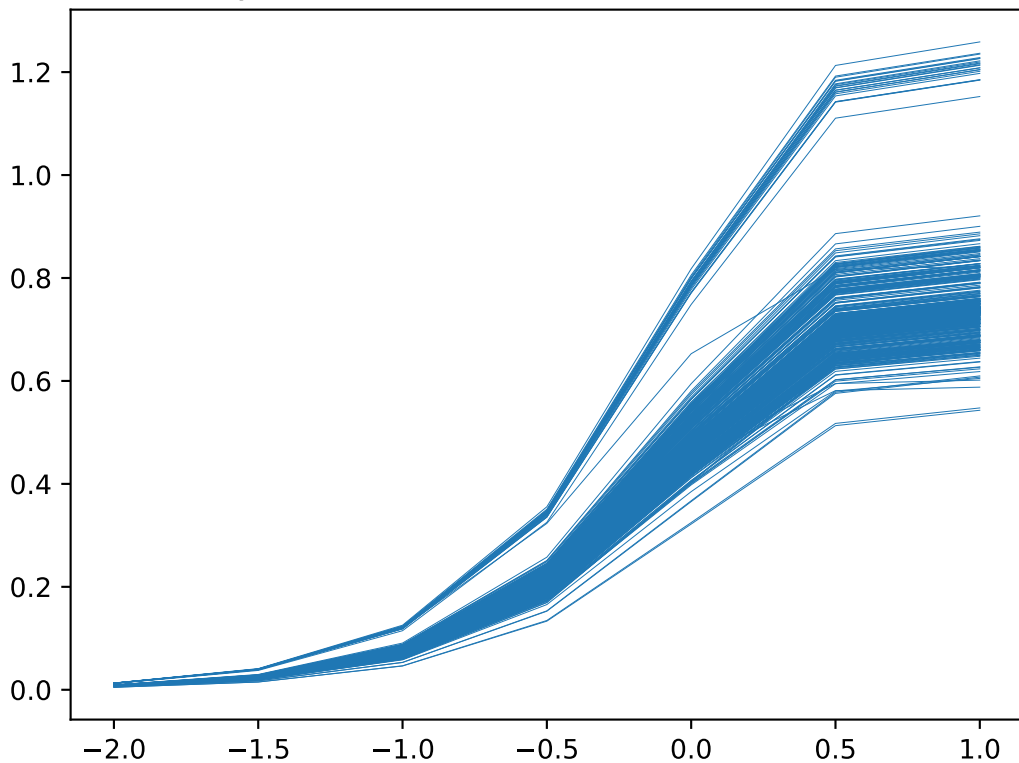
Dynamic Ricci Curvature for Geodesic 0.1
